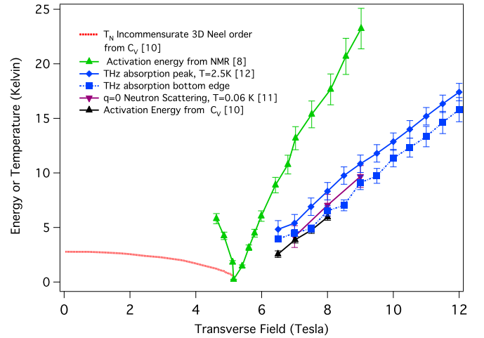
FIG. 4. Phase diagram and energy scales of the Ising chain system \text{CoNb}_2\text{O}_6 as a function of transverse field. Energy scales from different experimental probes as well as the transition temperature of the 3D incommensurate Néel order are given. The transition is to a state with ferromagnetic chains that are ordered antiferromagnetically in the b direction. On the paramagnetic side of the transition, one can see an excellent agreement between various spectroscopic probes (THz absorption [12] and inelastic neutron scattering [11] and heat capacity [10]). In contrast one can see clearly that the gap extracted from the temperature dependence of the NMR spin relaxation time is approximately twice as large [8].
