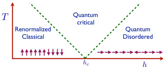
FIG. 1. Crossover phase diagram of the Ising chain in a transverse field h . There is a quantum critical point at T = 0 and h = h_c [for the Hamiltonian in Eq. (2.1), h_c = 1 ] between a ferromagnetic ( h < h_c ) which breaks the Ising symmetry, and a paramagnetic phase. This paper focuses on the quantum disordered regime above the paramagnetic phase for h > h_c . The other regimes were described in Ref. [8].
