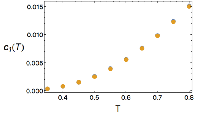
FIG. 2. c_1(T) for h = 1.5 and several temperatures. The thermodynamic limit result (blue dots, barely visible) is seen to be in good agreement with the extrapolation of numerical results for L = 192 and 0.1 \leq \eta \leq 0.115 (yellow dots).
